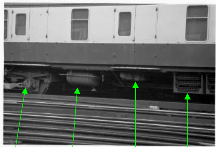
Trailer bogie, Main Reservoir, DH 16 Air compressor, No.2 bank of Grids Photo: David Smith
